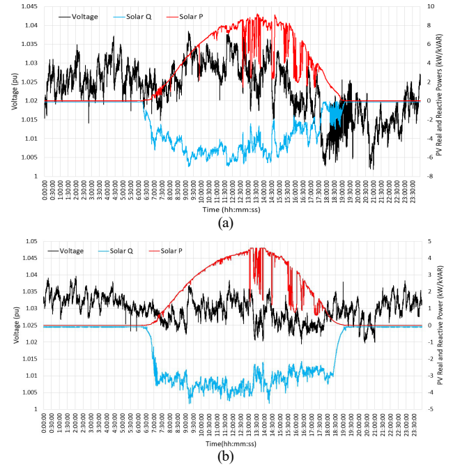
Figure 3: Local voltage, PV inverter real and reactive power over 24 hours under Volt/Var mode (a) 10 kVA, (b) 6 kVA.
