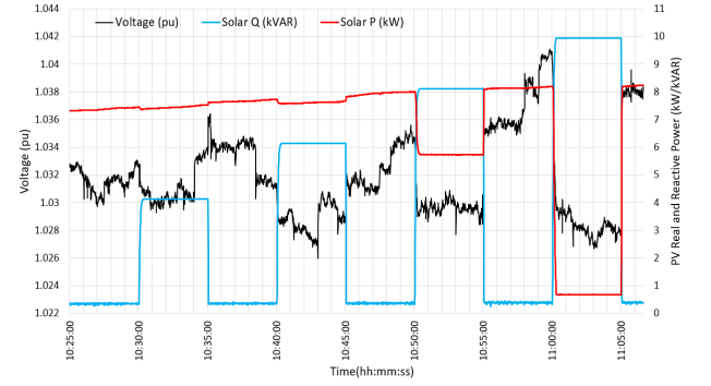
Fig. 6: Direct reactive power dispatch from 10 kVA inverter.
