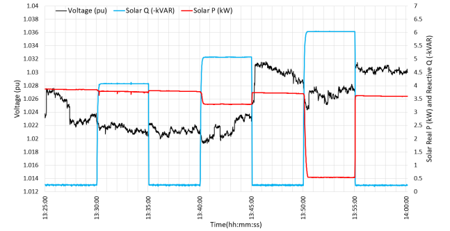
Fig. 7: Direct reactive power dispatch from 6 kVA inverter.
