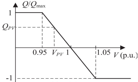
Figure 1: Typical Volt/VAR Control Curve.
