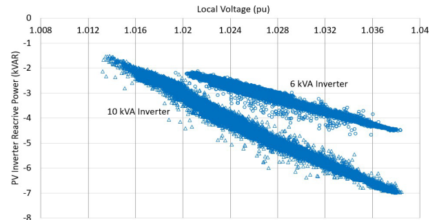
Figure 4: PV inverter reactive power as function of local voltage.
