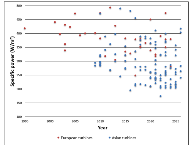
Fig.2. Specific power tendency of installed offshore wind turbines (1995-2026). Own elaboration.
