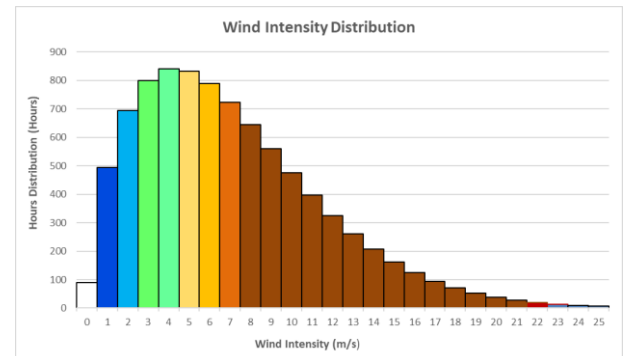
Fig.4. Wind intensity distribution graph.
