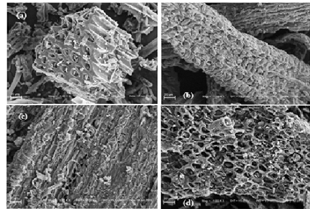
Fig.3. SEM images at 1000x magnification for (a) commercial activated carbon CAC, (b) carbon C/60, (c) carbon C/05, and (d) activated carbon AC/H 3 PO 4
