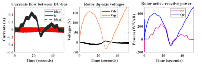
(a) DC-Bus currents (b) Rotor Voltages (c) Rotor active-reactive power Fig. 12. DC-bus currents, rotor voltages, and powers
