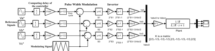
Fig. 4. Three-phase inverter system with delay compensation
