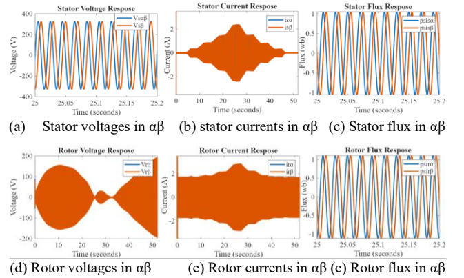
Fig. 9. Stator and Rotor voltages, currents, and flux responses
