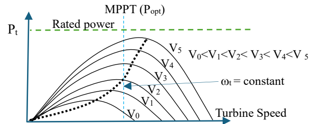
Fig. 6. Wind turbine characteristic for maximum power extraction
