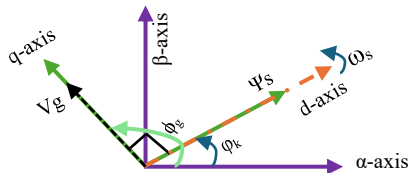
Fig. 5. Reference frame orientation with Stator flux
