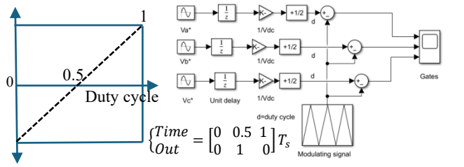
a) Duty cycles
