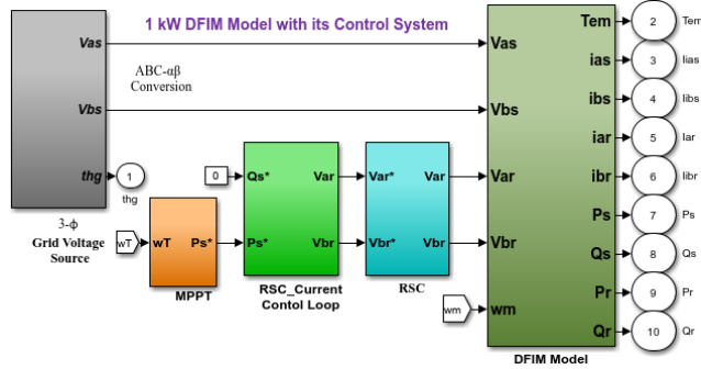
Fig. 7. DFIM and RSC controller under MPPT algorithm
