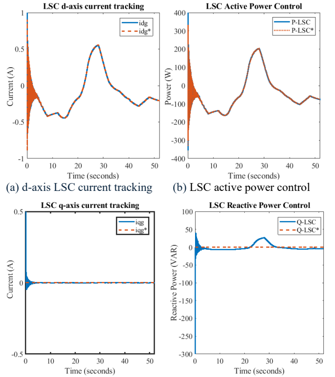
(c) q-axis LSC current tracking (d) LSC reactive power control Fig. 14. Line side converter active-reactive power control
