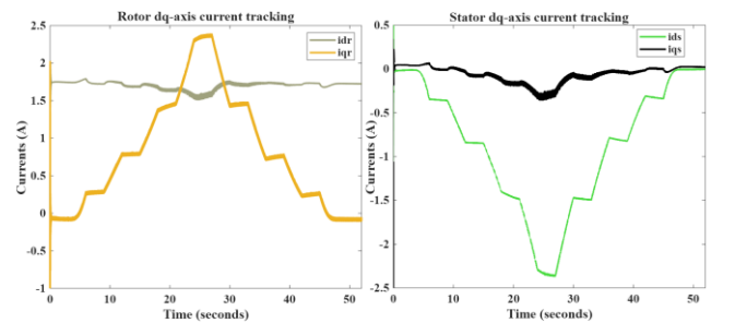
Fig. 10. Rotor and stator dq-currents
