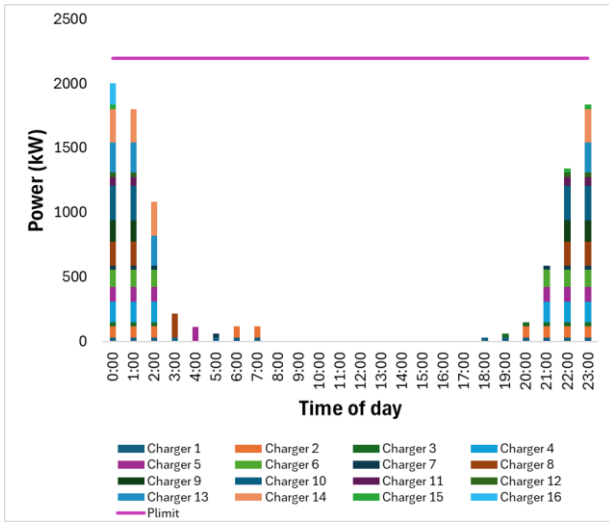
Fig. 5. Daily charging power profile by charger with grid power limit.
