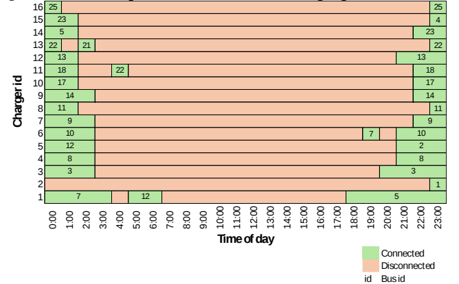
Fig. 4. Temporal evolution of charger usage and bus assignment throughout the day
